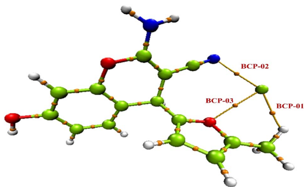
Fig. 11 QTAIM analysis results of the CFN- \text{Ca}^{2+} complex.
