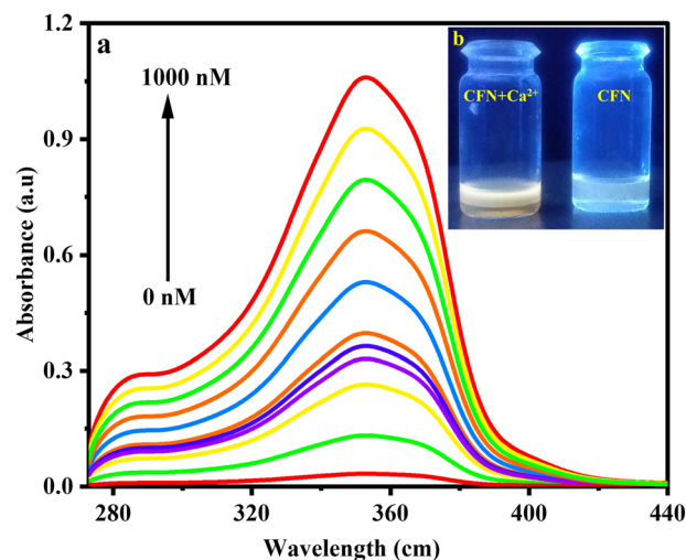
Fig. 6 UV-Vis absorption spectra generated after the concomitant addition of \text{Ca}^{2+} (0–1000 nM) to aqueous solution (water : DMF = 9 : 1, v/v) of the CFN sensor (a) and photographs showing the visual colorimetric detection of \text{Ca}^{2+} under a 365 nm UV lamp (b).
