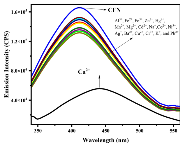
Fig. 5 Fluorescence emission spectra of the CFN sensor scanned in the presence of a range of competing metal ions. The emission spectra were obtained in \text{H}_2\text{O}:\text{DMF} (9 : 1, v/v; 30 \mu\text{M} ; \lambda_{\text{exc}} = 330 nm; S_w = 3/3 ).
