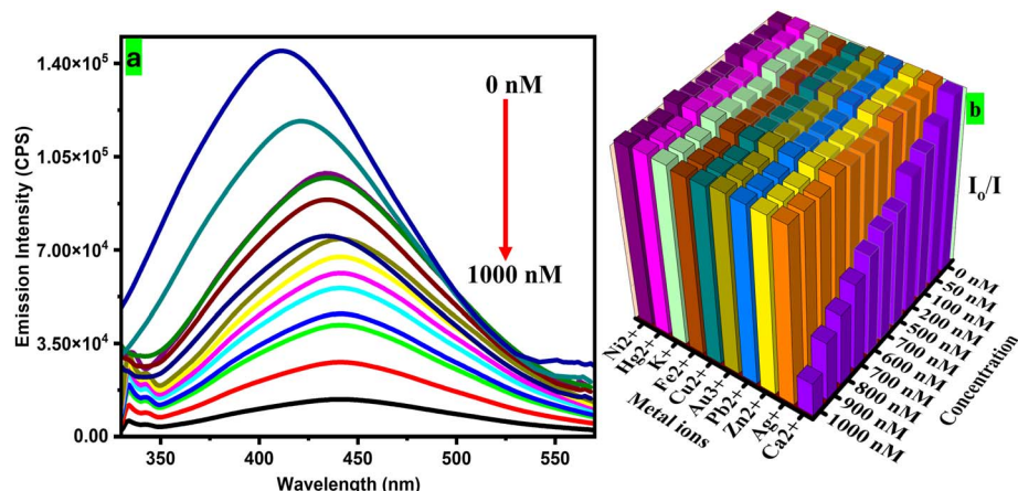
Fig. 7 Fluorescence emission spectra (a) and the corresponding 3D Stern–Volmer plot (b) of the CFN sensor upon the consistent addition of Ca 2+ (0–1000 nM) in aqueous solutions (H 2 O : DMF = 9 : 1, v/v).
