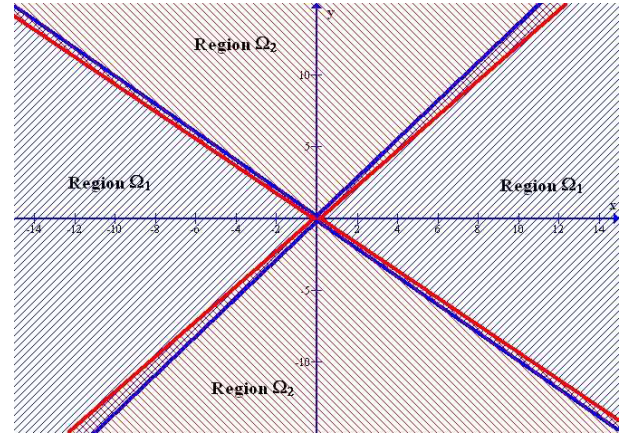
Fig. 1. Representation of regions \Omega_1 and \Omega_2
