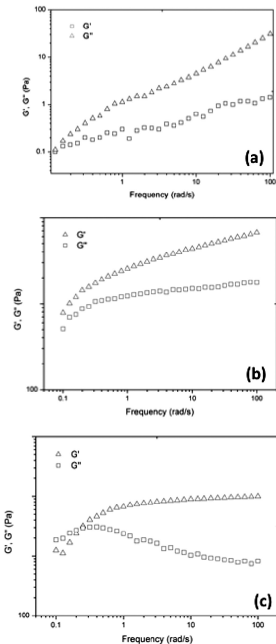
Figure 3. Elastic ( G' ) and viscous ( G'' ) modulus as a function of the frequency (rad/s) at 35°C for formulations containing: (a) 18% poloxamer; (b) 18% poloxamer + 1% hyaluronic acid, and; (c) 18% poloxamer + 1% hyaluronic acid + 1% microparticles
