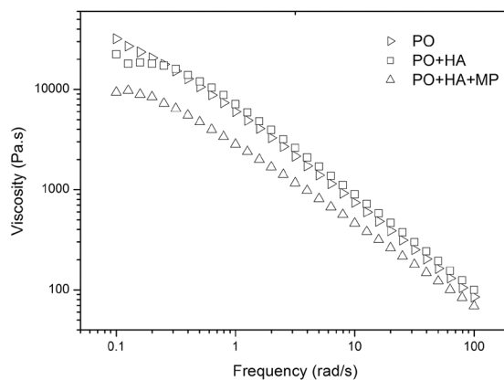
Figure 5. Viscosity vs. frequency curves at 35°C for the three formulations listed in Table 2
