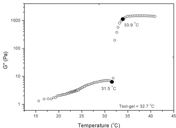
Figure 1. Sol-gel transition temperature ( T_{\text{sol-gel}} ) using 17.5% Poloxamer 407®
