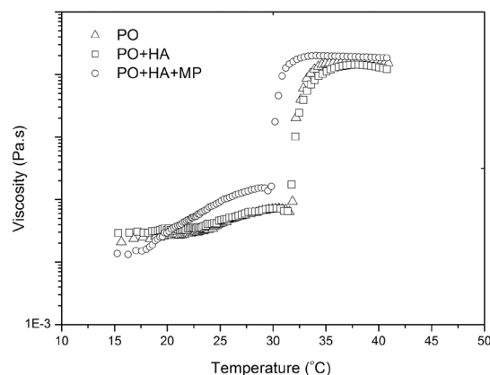
Figure 4. Viscosity vs. temperature curves for the three formulations listed in Table 2 at 1 rad/s
