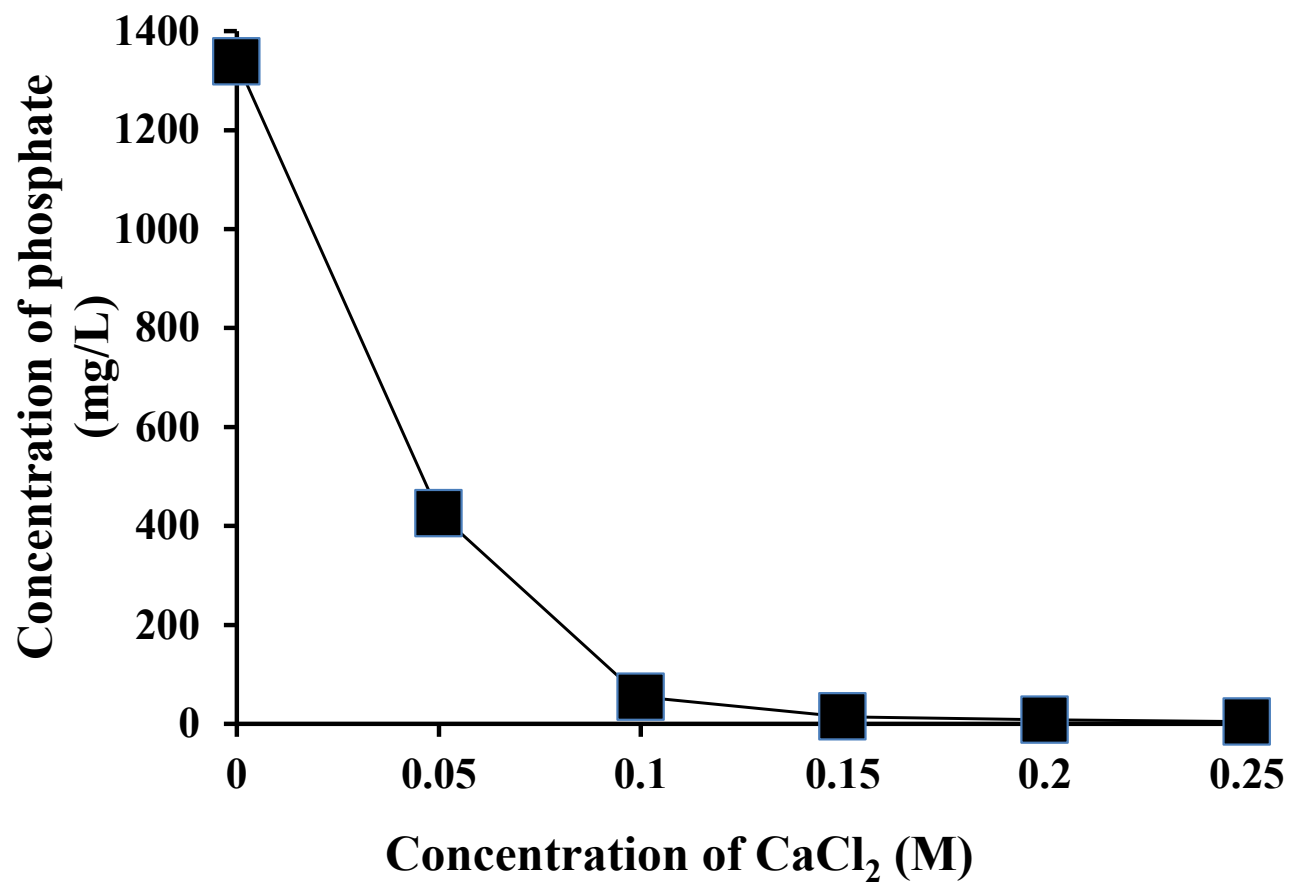
Figure 6.11. Supernatant concentrations of phosphate after \text{CaCl}_2 addition to the solution obtained by 1M NaOH leaching of Purolite FerrIX A33E resin after phosphate adsorption.
