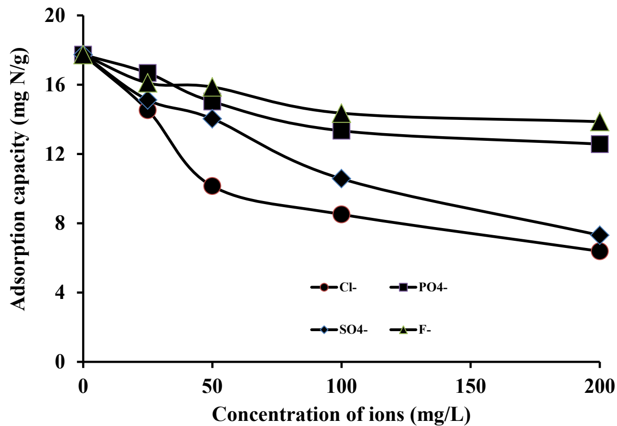
Figure 4.5. Influence of background ions on the adsorption of nitrate by Purolite A520E (initial nitrate concentration 20 mg N/L and adsorbent dose 1g/L).
