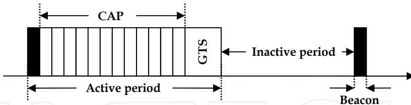
Fig. 6. Superframe structure in beamed mode IEEE 802.15.4 MAC.
