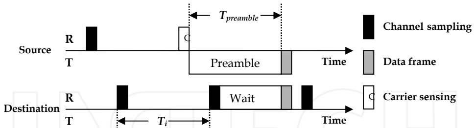
Fig. 7. Basic operation of unsynchronised Berkeley MAC.
