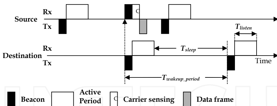
Fig. 2. A synchronous periodic wake-up scheme.
