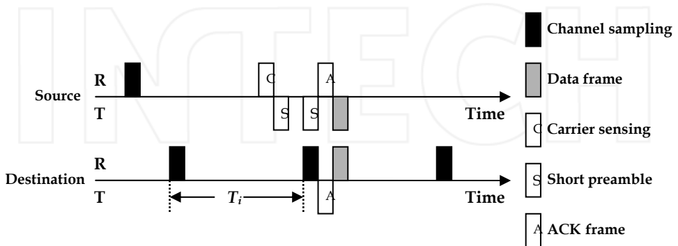
Fig. 9. Basic operation of unsynchronised X-MAC.
