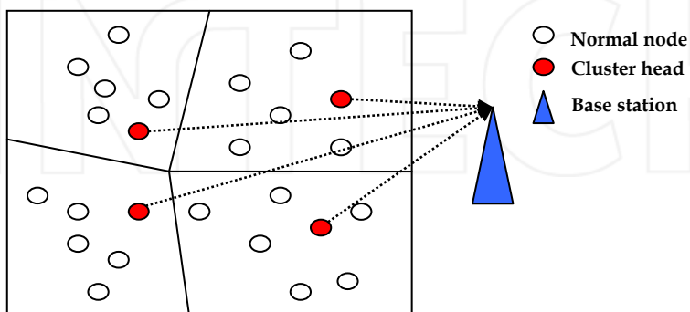
Fig. 3. Clustered LEACH MAC architecture.
