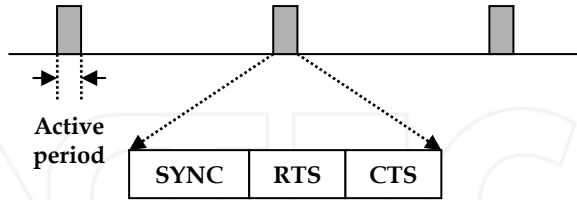
Fig. 4. S-MAC synchronous periodic wake-up scheme.
