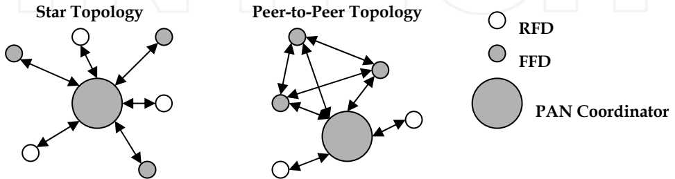
Fig. 5. Topology configurations supported by IEEE 802.15.4 standard.
