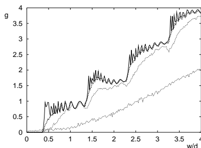
Figure 3: Mean conductance of ensemble of disordered waveguides. As for Fig. 2, but with disorder at 0%, 6.67%, 13.3%, 26.67% from top to bottom.
