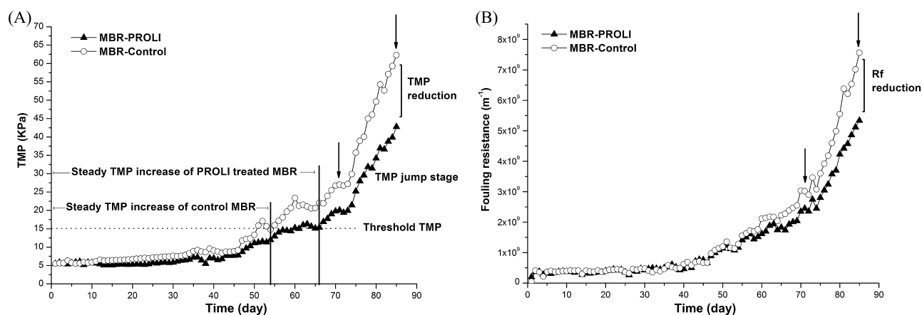
Fig. 2. The effect of PROLI-NONOate treatment on the formation of biofilms from the commencement of MBR operation. The horizontal dashed line indicates the threshold TMP between the low pressure TMP stage and the TMP jump stage. The vertical lines show when PROLI-treated MBR and control MBR reached the TMP jump stage. The downward pointing arrows indicate the times at which membrane and sludge samples were collected and analysed to determine TMP (A) and R_f (B). The R_f values were determined after the daily PROLI NONOate treatment.
