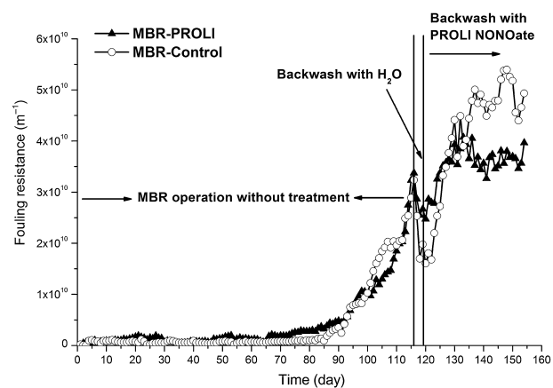
Fig. 1. The effect of PROLI-NONOate backwashing treatment on pre-established biofilm at high TMP. Fouling was quantified by determining the resistance of the membrane to the passage of water. The vertical lines separate the experiment into three phases: normal MBR operation, backwashing with dH 2 O (distilled water) and backwashing with PROLI NONOate. The R_f values were determined after daily backwashing.
