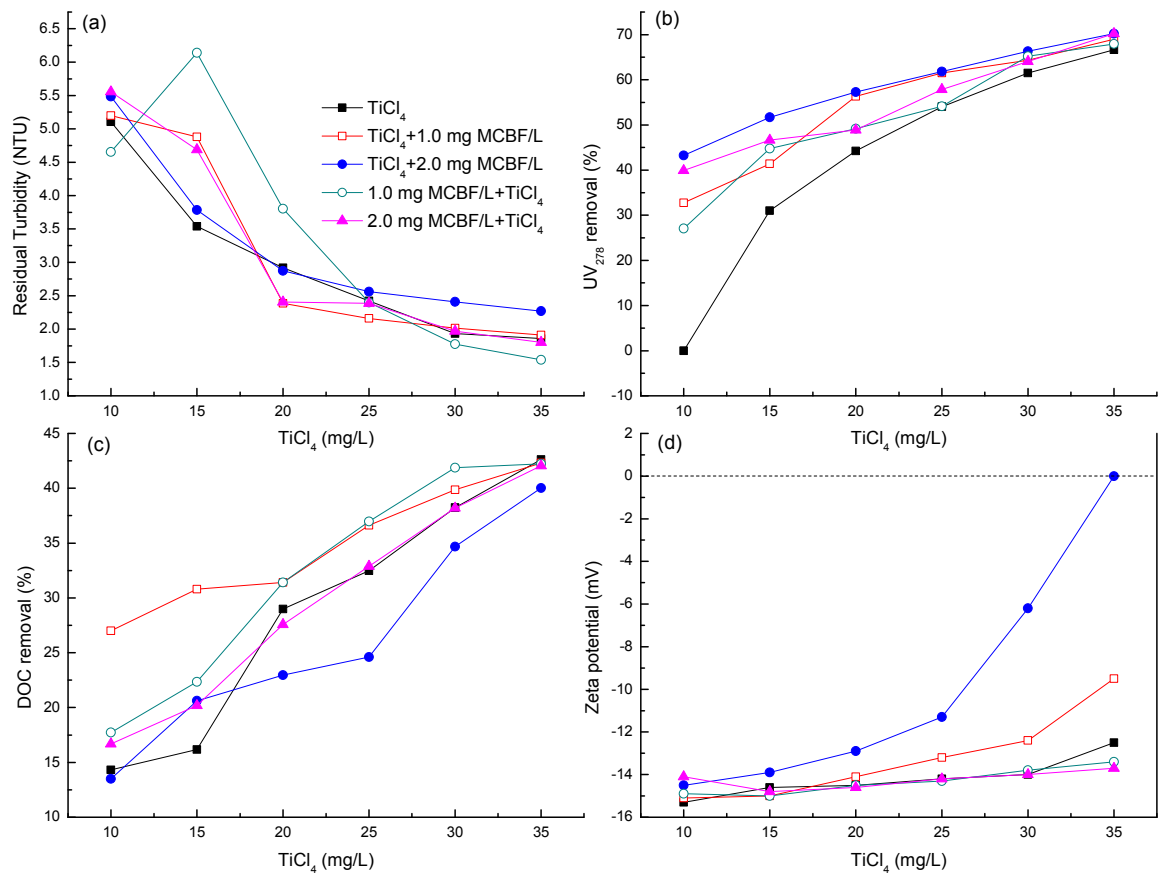
Fig. 3 Effect of MCBF dose and dosing sequence on: residual turbidity (a), UV_{278} removal (b), DOC removal (c) and zeta potential (d) for FA simulated water treatment
