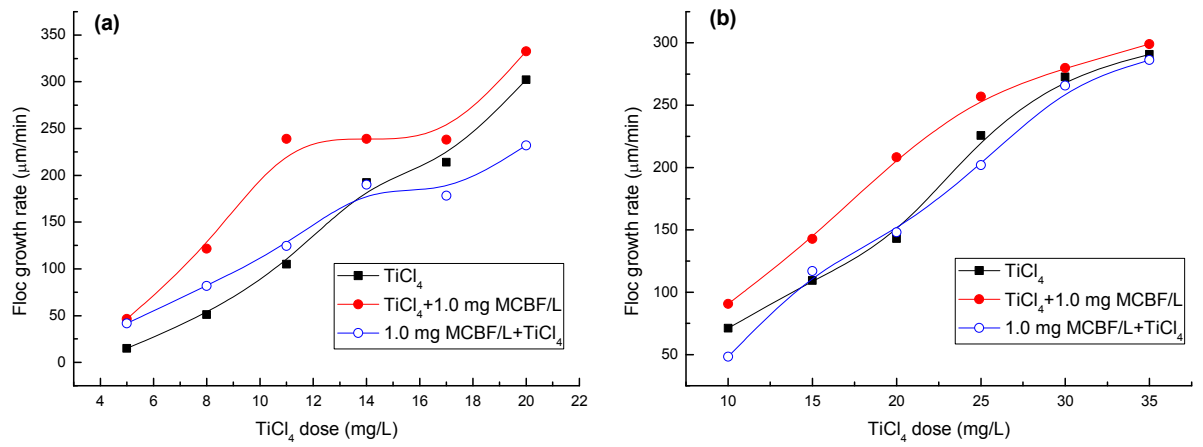
Fig. 4 Change in floc growth rate vs. coagulant dose with different coagulants for simulated water treatment: HA (a) and FA (b)
