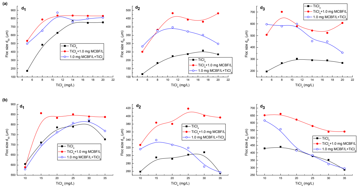
Fig. 5 Variation of floc size d_1 , d_2 and d_3 as a function of coagulant dose with different coagulants for simulated water treatment: HA (a) and FA (b)
