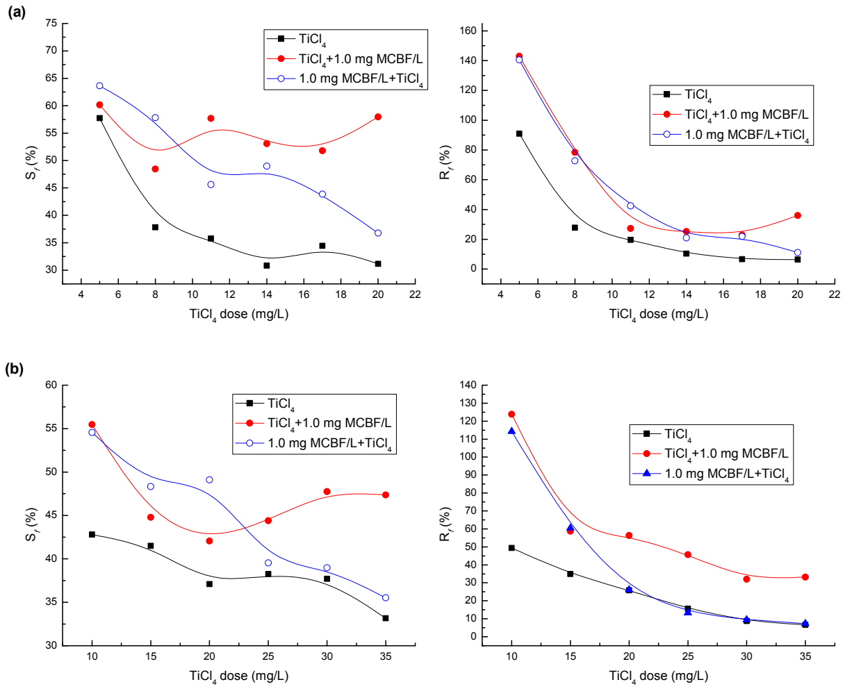
Fig. 6 Change in S_f and R_f vs. coagulant dose with different coagulants for simulated water treatment: HA (a) and FA (b)
