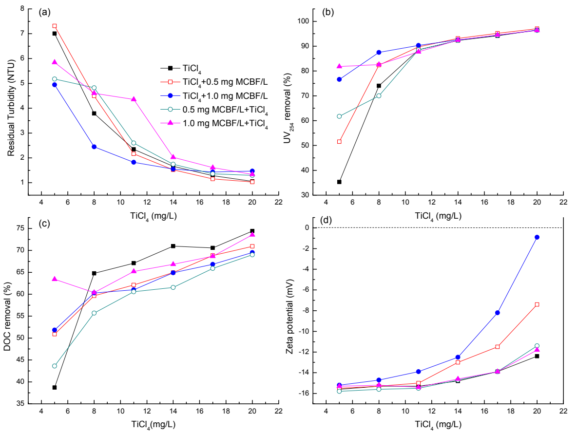
Fig. 2 Effect of MCBF dose and dosing sequence on: residual turbidity (a), \text{UV}_{254} removal (b), DOC removal (c) and zeta potential (d) for HA simulated water treatment
