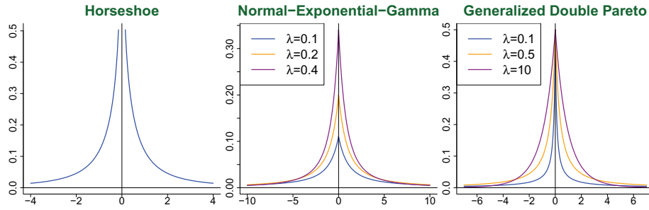
FIG 12. Left panel: the standard Horseshoe density function. Middle panel: three standard Normal-Exponential-Gamma density functions with varying shape parameter \lambda . Right panel: three standard Double Generalized Pareto density functions with varying shape parameter \lambda .
