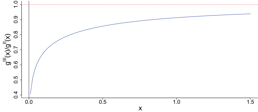
FIG 4. Plot of g^{III}(x)/g^{II}(x) for the functions g^{II} and g^{III} defined by (2.6).
