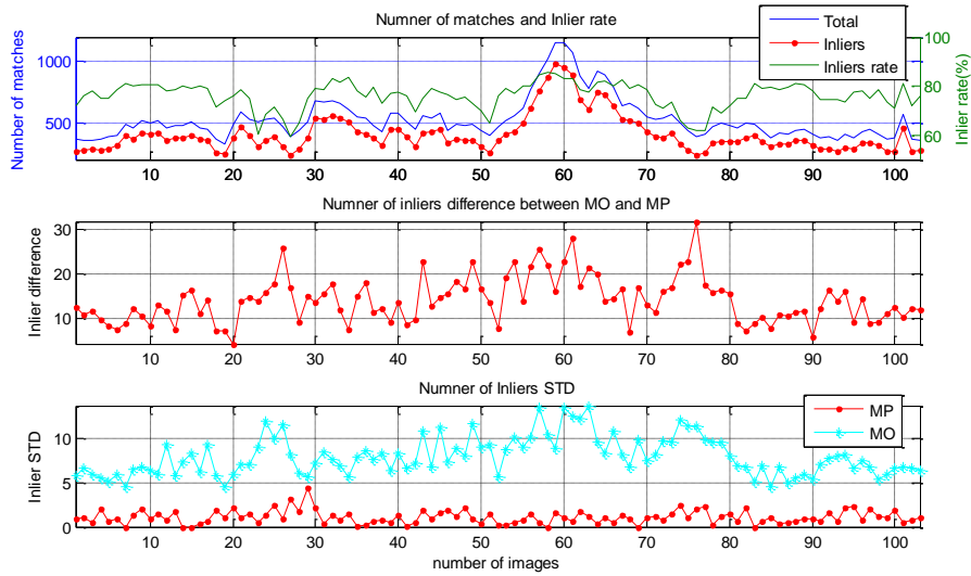
Figure 5. Number of inliers in visual odometry tests
