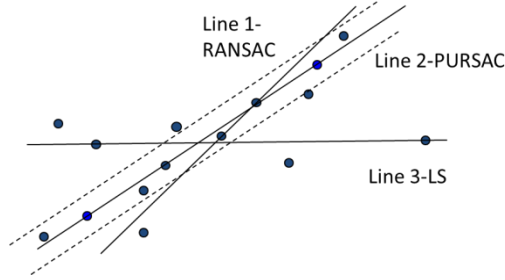
Figure 1. Line fitting results by RANSAC (Line 1) , PURSAC (Line 2) and least square (Line 3).
