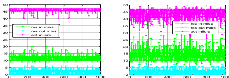
Figure 3. 1000 runs Monte Carlo test results with PURSAC and RANSAC.
