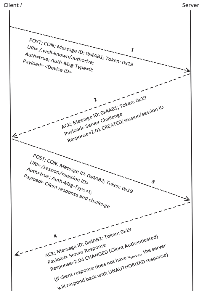
Figure 7.2: Four-way Authentication Handshake
