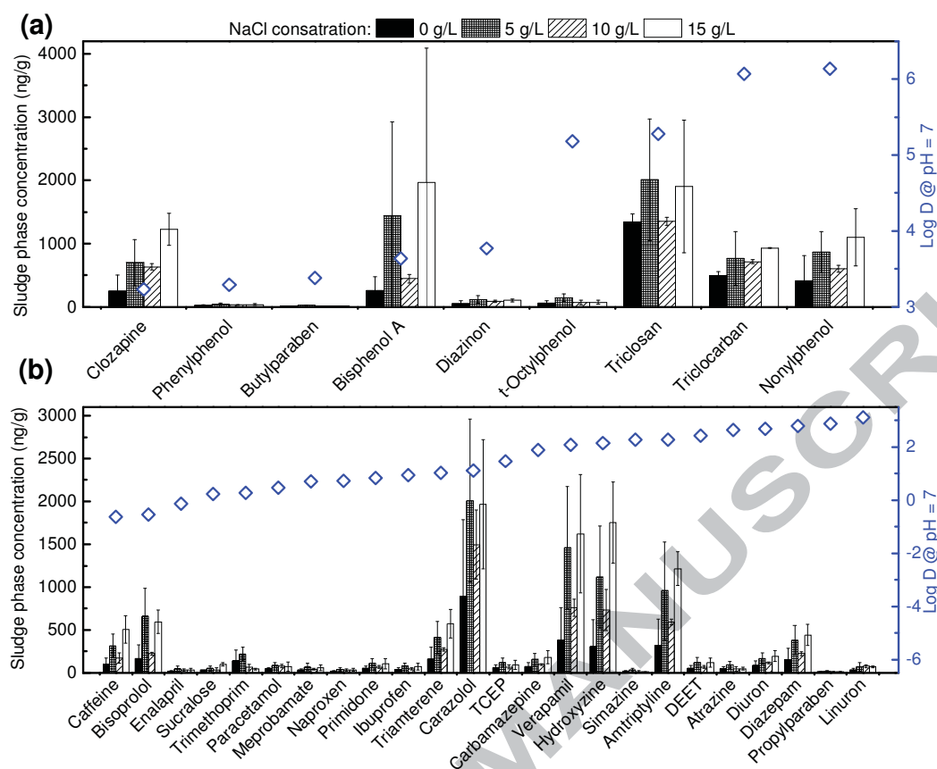
Figure 5: Effect of salinity build-up in the bioreactor on TrOC accumulation in the sludge during AnMBR operation. Salinity build-up in the bioreactor was simulated by gradually increasing the feed NaCl concentration from 0 to 15 g/L. To allow microbial acclimatization to the salinity stress, the influent salt salinity was maintained at 5, 10, and 15 g/L NaCl for two weeks. Error bars represent the standard deviation of two measurements (once per week) at each salinity condition.
