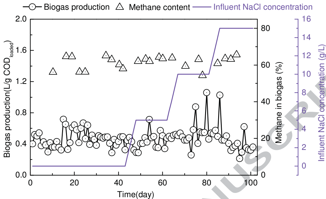
Figure 2: Effect of salinity build-up in the bioreactor on biogas production and its methane content during AnMBR operation. Salinity build-up in the bioreactor was simulated by increasing the feed NaCl concentration from 0 to 15 g/L. Experimental conditions are as described in the caption of Figure 1.
