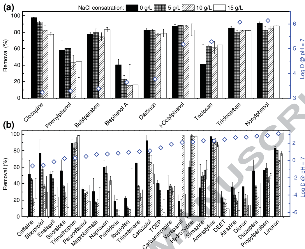
Figure 4: Effects of salinity build-up in the bioreactor on the removal of TrOCs by AnMBR treatment. The 33 TrOCs investigated could be grouped into hydrophobic ( \text{Log } D > 3.2 at pH 7) and hydrophilic ( \text{Log } D < 3.2 at pH 7). Salinity build-up in the bioreactor was simulated by gradually increasing the feed NaCl concentration from 0 to 15 g/L. To allow microbial acclimatization to the salinity stress, the influent salt salinity was maintained at 5, 10, and 15 g/L NaCl for two weeks. Error bars represent the standard deviation of two measurements (once per week) at each salinity condition.
