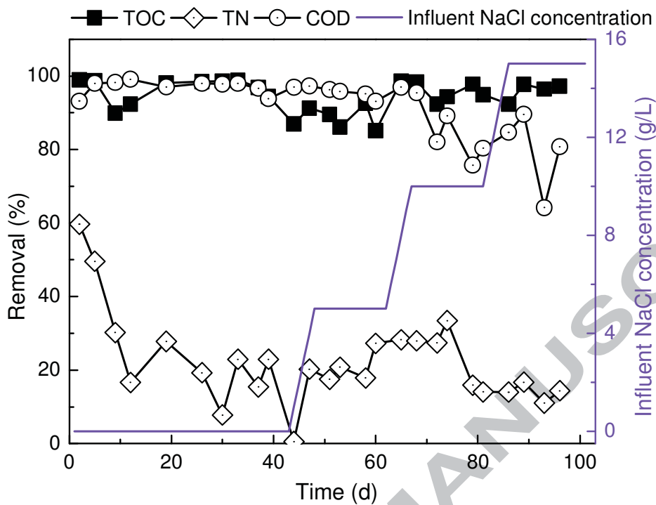
Figure 1: Effects of salinity build-up in the bioreactor on the removal of bulk organic matter (i.e. TOC, TN, and COD) by AnMBR. Salinity build-up in the bioreactor was simulated by increasing the feed NaCl concentration from 0 to 15 g/L. Experimental conditions: initial MLSS = 16 g/L; HRT = 5 d; mixed liquor pH = 7 \pm 0.1 (adjusted by sodium acetate); temperature = 35 \pm 1 °C.
