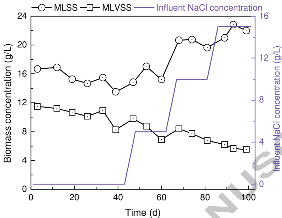
Figure 3: Effect of salinity build-up in the bioreactor on biomass concentration during AnMBR operation. Salinity build-up in the bioreactor was simulated by increasing the feed NaCl concentration from 0 to 15 g/L. Experimental conditions are as described in the caption of Figure 1.
