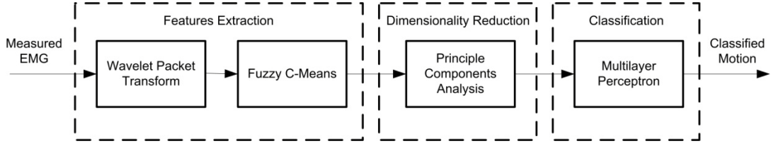
Fig. 2. The proposed MES recognition system.
