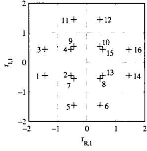
(a) Constellation at receiver 1.
