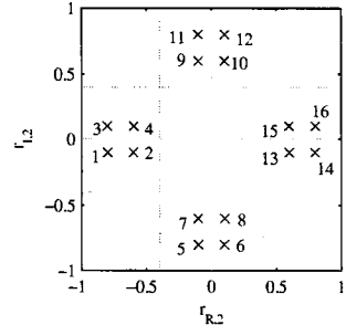
(b) Constellation at receiver 2.
