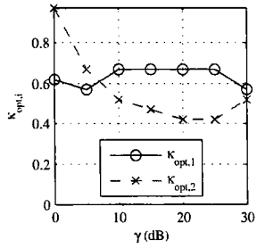
(l) Optimal normalized clip levels
