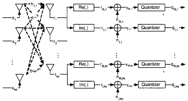
Fig. 1. MIMO system with quantization
