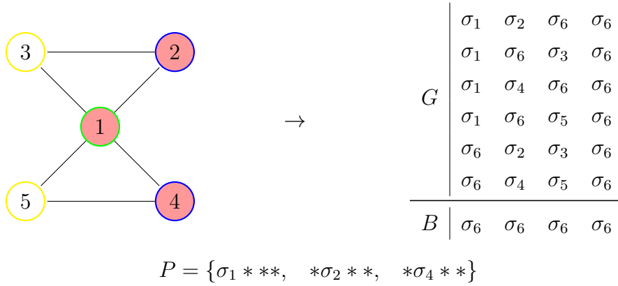
Figure 3: An example of the reduction used in Lemma 3.15 with k = 3 . The vertex cover is highlighted in red, and the correspond set of patterns is shown. Note the difference with the reduction in Lemma 3.11, here the position encodes the coloring and the symbols encode the edges, whereas previously the string more directly encode the graph.
