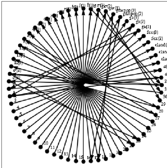
Illustration 39: Exogenous equations
