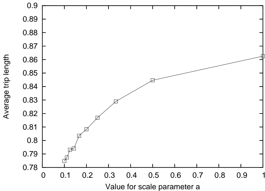
Figure 4.19: Simulated effect of activity distribution on trip length.
