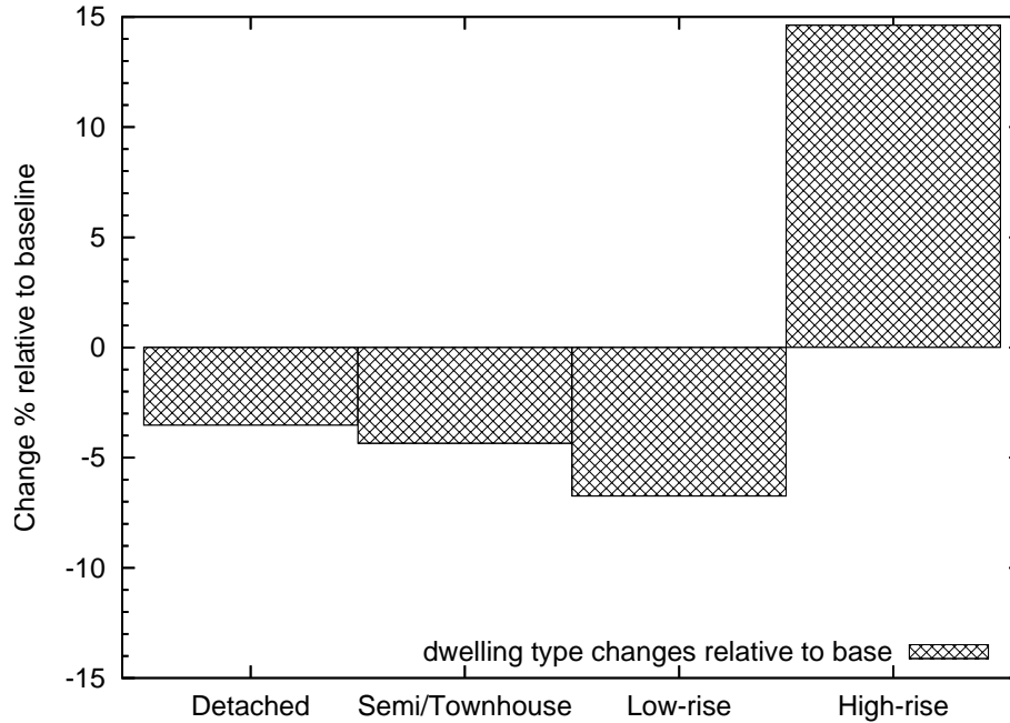
Figure 9.68: Scenario 10: Change in dwelling mix, compared to baseline scenario. Note that these are absolute percentages, so a reported 1% decline indicates that the proportion of all dwellings of that dwelling type is 1% lower.
