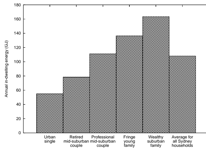
Figure 7.17: In-dwelling energy use per household for the example households.
