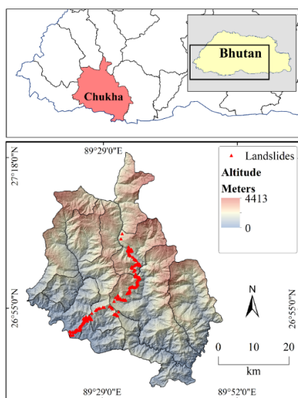
Figure 2. Study area, showing the altitude and landslide data points.
