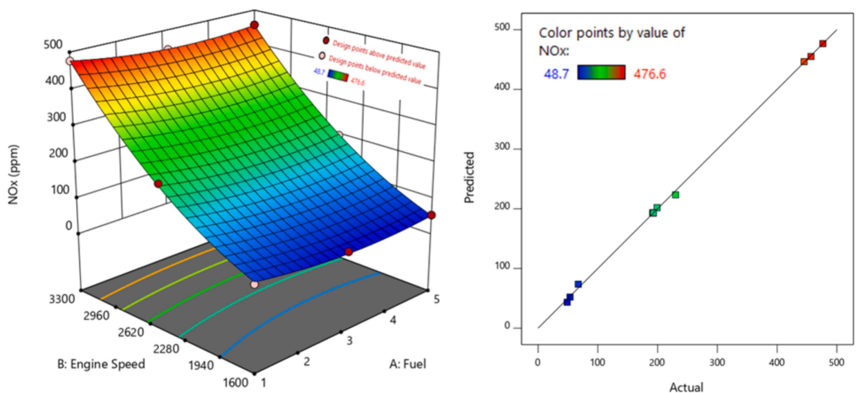
Fig. 17. (a) Response surface of NO x , (b) Comparison of actual and predicted NO x values.
