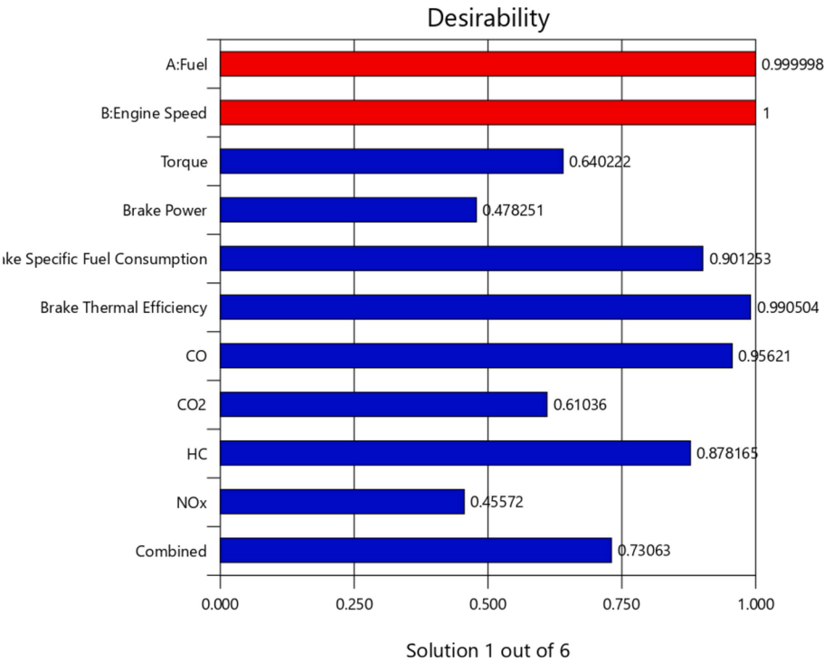
Fig. 19. Desirability chart.
