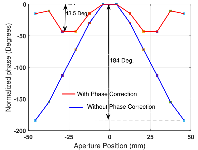
FIGURE 7. Electric-field ( E_y ) phase distribution along the x-axis before and after phase correction.
