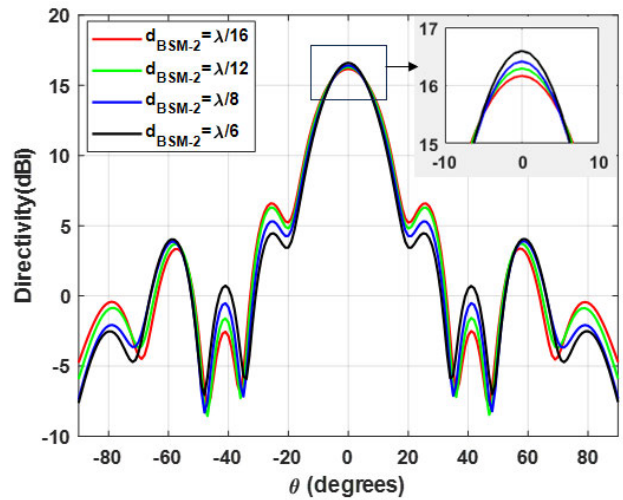
FIGURE 12. Directivity pattern in elevation plane of the beam steering antenna in the broadside direction for inter-spacing variation between PC-BSM-1 and BSM-2 from \lambda/16 to \lambda/6 .
