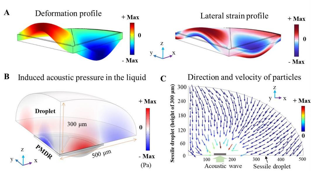
Fig. 2 Theoretical simulation of the PMDR resonance for acoustic enrichment and mass sensing. (A). Simulation of the deformation profile and lateral strain profile of the transverse (2, 0) mode excited in a circular diaphragm with the diameter of 560 \mu\text{m} . (B) Sectional view of the induced acoustic pressure by the resonance of PMDR in a sessile droplet. (C) Particle trace simulation model shows the direction and velocity of particles in a droplet under the treatment of acoustic radiation force (applied at the position of the bold grey line), while the trajectory of particles is animated in Video S1 (Multimedia available online).
